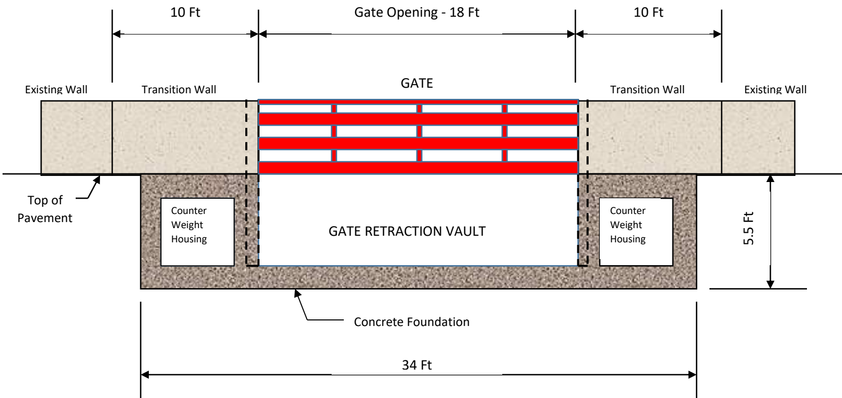
RESPONDER GATE – ELEVATION VIEW
